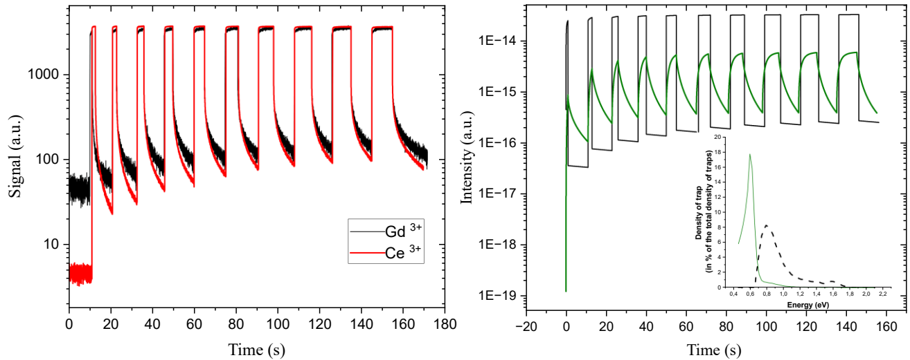
Figure 1 - (Left) RL graph for SiO 2 :Gd and SiO 2 :Ce at increasing exposure time, constant dose rate; (Right) RL modelization for increasing exposure time with two different densities of trap. The inset represents the two used densities of traps, with the same color code as the intensity.
