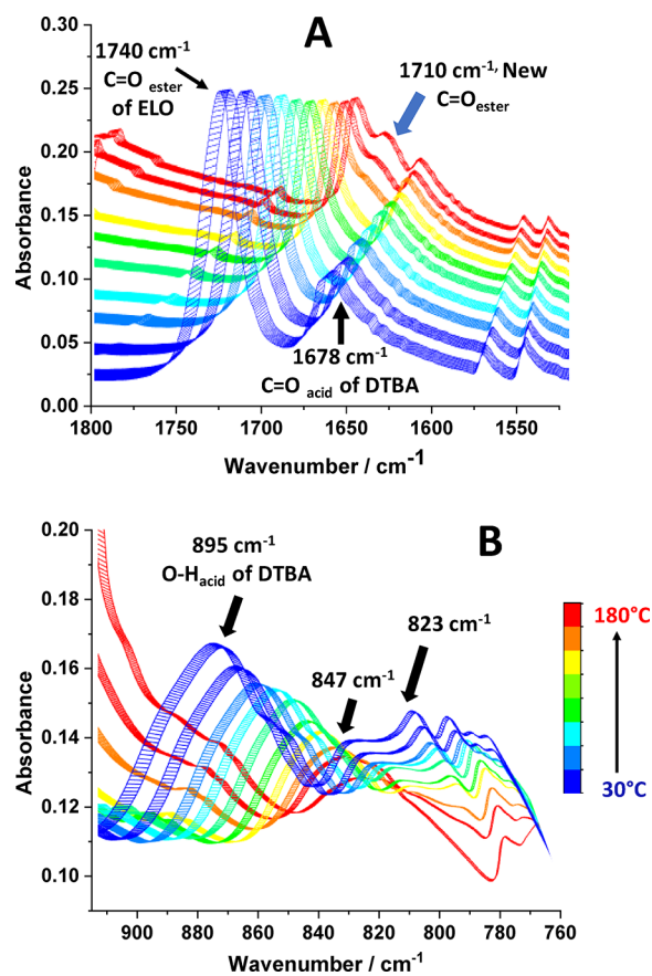
Figure 2. Evolution of FT-IR spectra of the ELO/DTBA mixture during heating from 30 to 180\text{ }^{\circ}\text{C} at 10\text{ }^{\circ}\text{C}\cdot\text{min}^{-1} . (A) Zoomed-in region of 1800\text{--}1525\text{ cm}^{-1} ; (B) zoomed-in region of 915\text{--}760\text{ cm}^{-1} .
