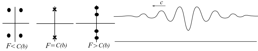
Figure 4. (left) (i\omega)^2 resonance for F near C(b) , and (right) shape of one of the two types of solitary waves for b < 1/3 , F < C(b) .
