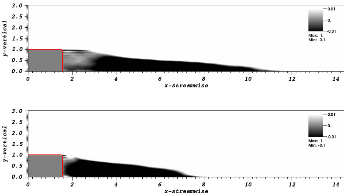
Figure 8: Mean streamwise velocity for the natural flow (top) and for the controlled flow, with U_{jet} = 1.5 and St_{jet} = 0.15 (bottom).
