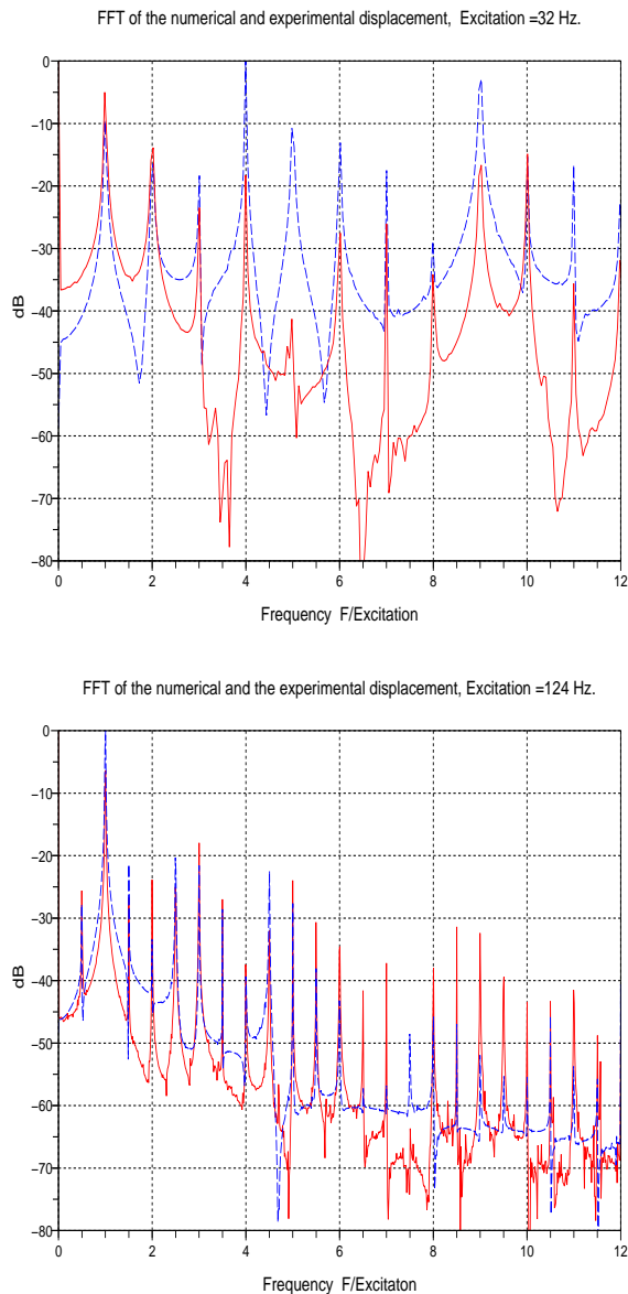
Figure 7: dashed line: FFT and the experimental displacements, solid line: FFT of the numerical displacements. Two different excitation: 32Hz and 124Hz
